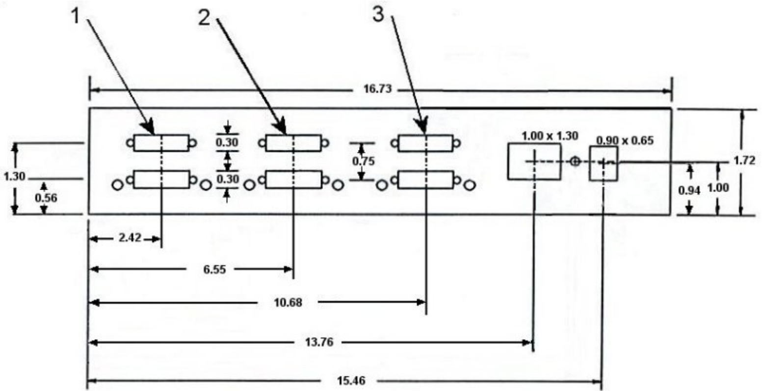
REAR VIEW DIMENSIONS IN INCHES
